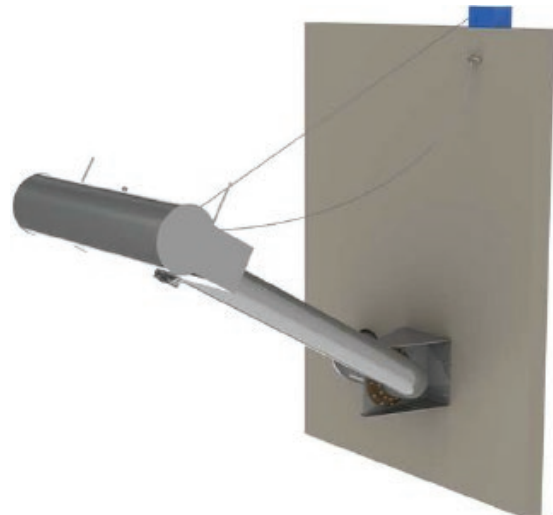
BioJet™ Floating Decanter with Winch
